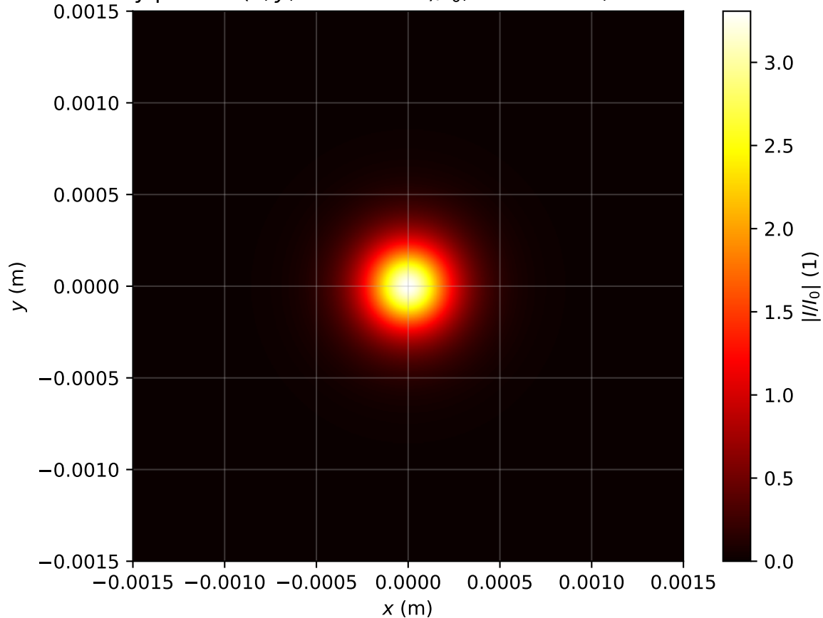
Intensity profile I(x, y, z = 3.901m)/I_0 , P_{in}=1.0P_{cr} , artificial time
